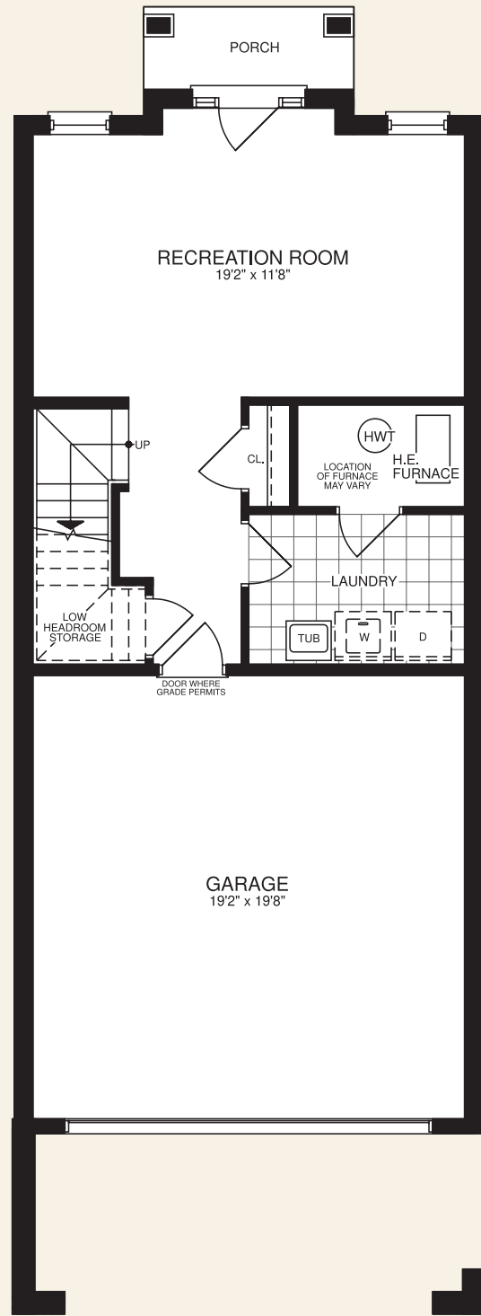
MAIN FLOOR ELEV. A
