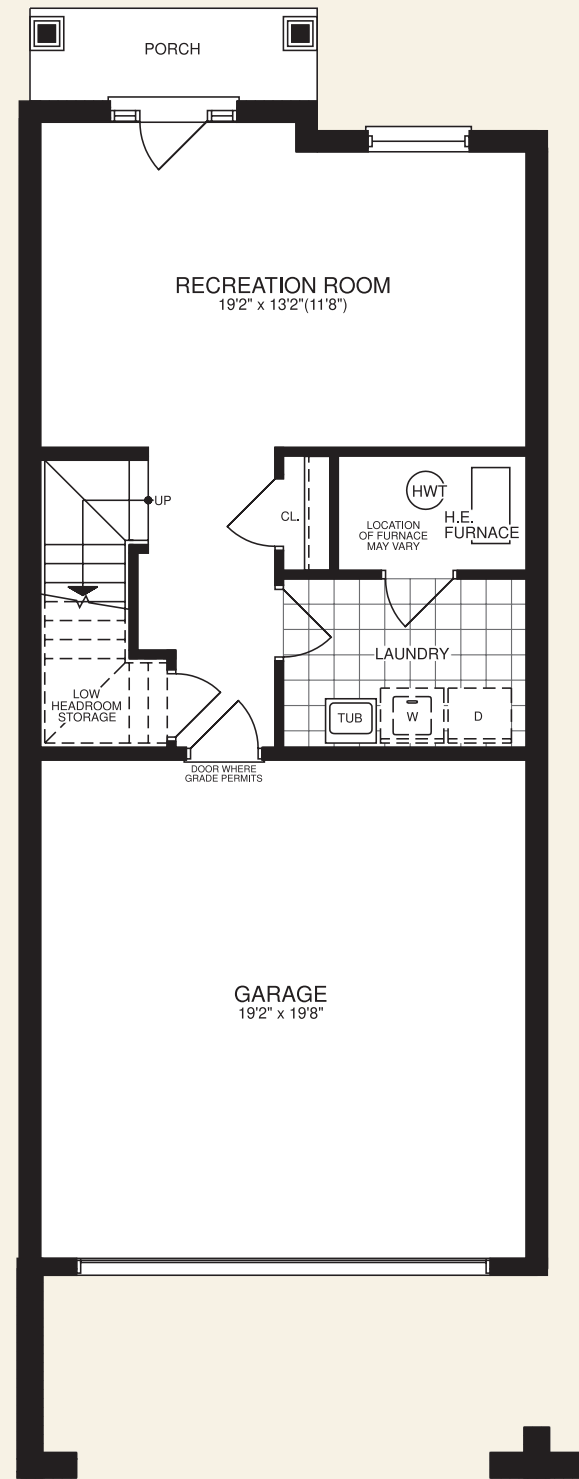
MAIN FLOOR ELEV. D
