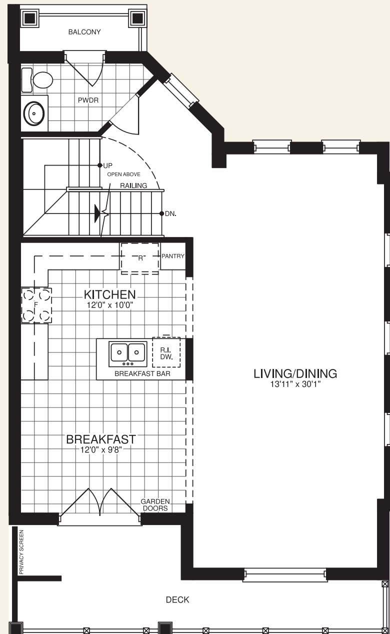
FIRST FLOOR ELEV. A
